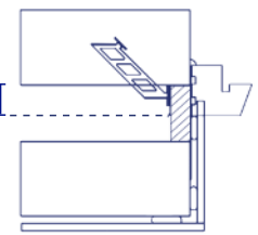
Staggered jamb
