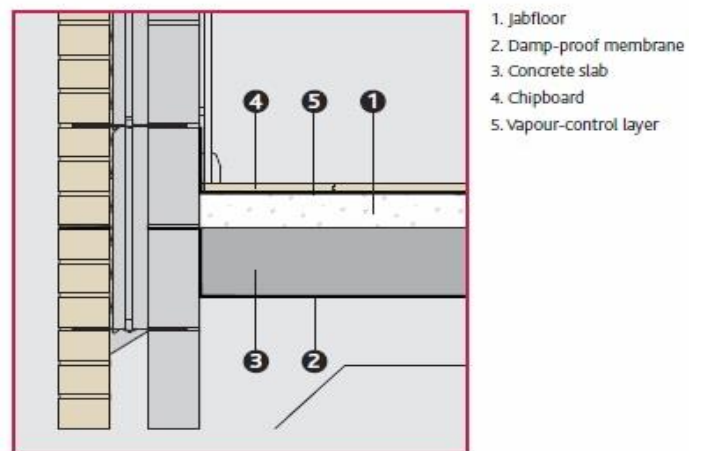
Damp-proof membrane below concrete slab
